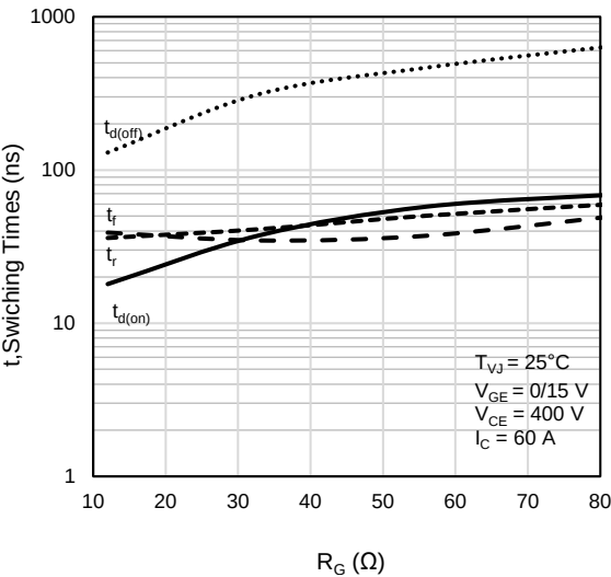
Figure 9: Switching Times vs. Gate Resistor
