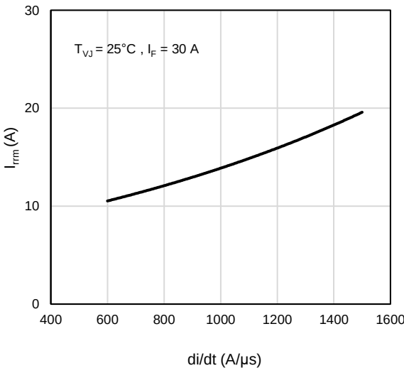
Figure 22: Reverse Recovery Current vs. Diode Current Slope
